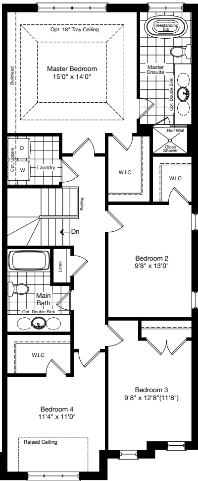
SECOND FLOOR ELEVATION B
