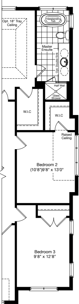
PARTIAL SECOND FLOOR ELEVATION A CORNER UPGRADE
