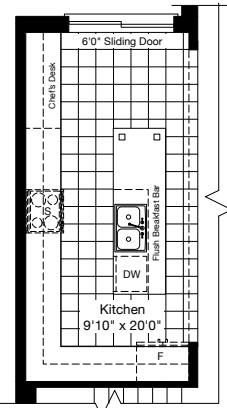
PARTIAL OPTIONAL KITCHEN LAYOUT
