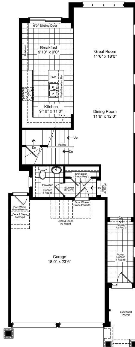
GROUND FLOOR ELEVATION B
