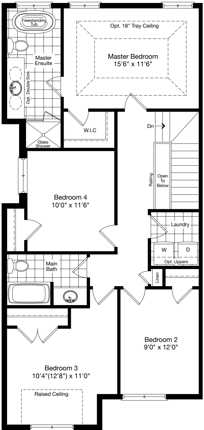
OPTIONAL SECOND FLOOR W/4 BEDROOMS ELEVATION A
