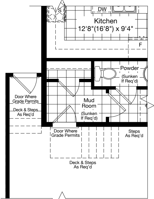
PARTIAL GROUND FLOOR ELEVATION A & B WHEN PAIRED WITH TH-01
