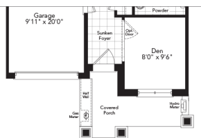
Partial Ground & Optional Ground Floor Elevation B
