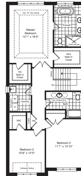
Upper Floor Elev. 'A' End
