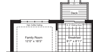
Partial Main Floor Elev. 'A' End LOB Condition
