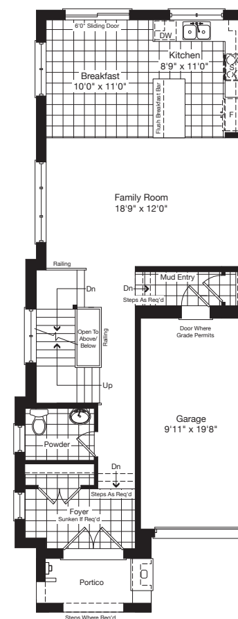
Main Floor Elev. 'A' Corner
