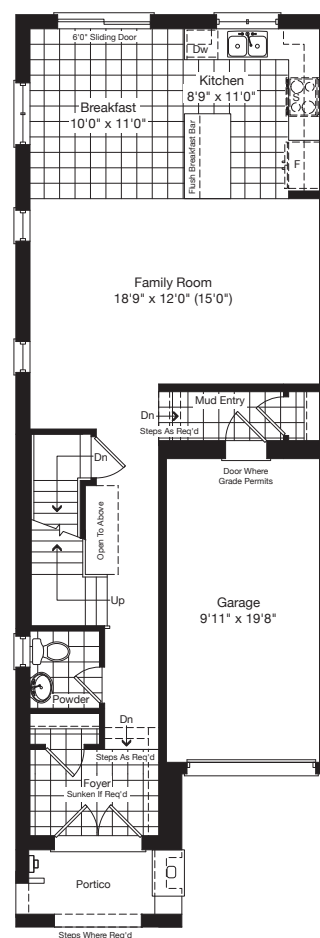
Main Floor Elev. 'A' End
