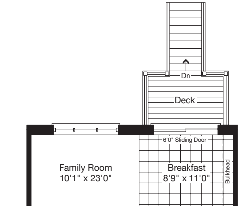
Partial Main Floor Elev. 'A' LOB Condition
