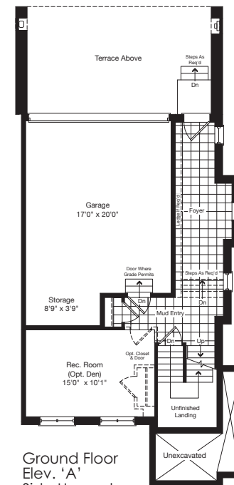
Ground Floor Elev. 'A' End
