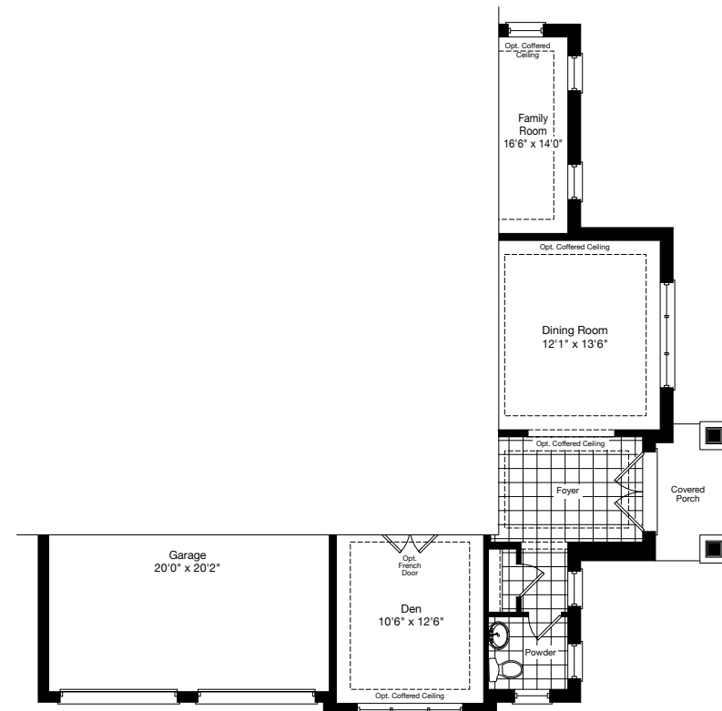
PARTIAL GROUND FLOOR ELEVATION B
