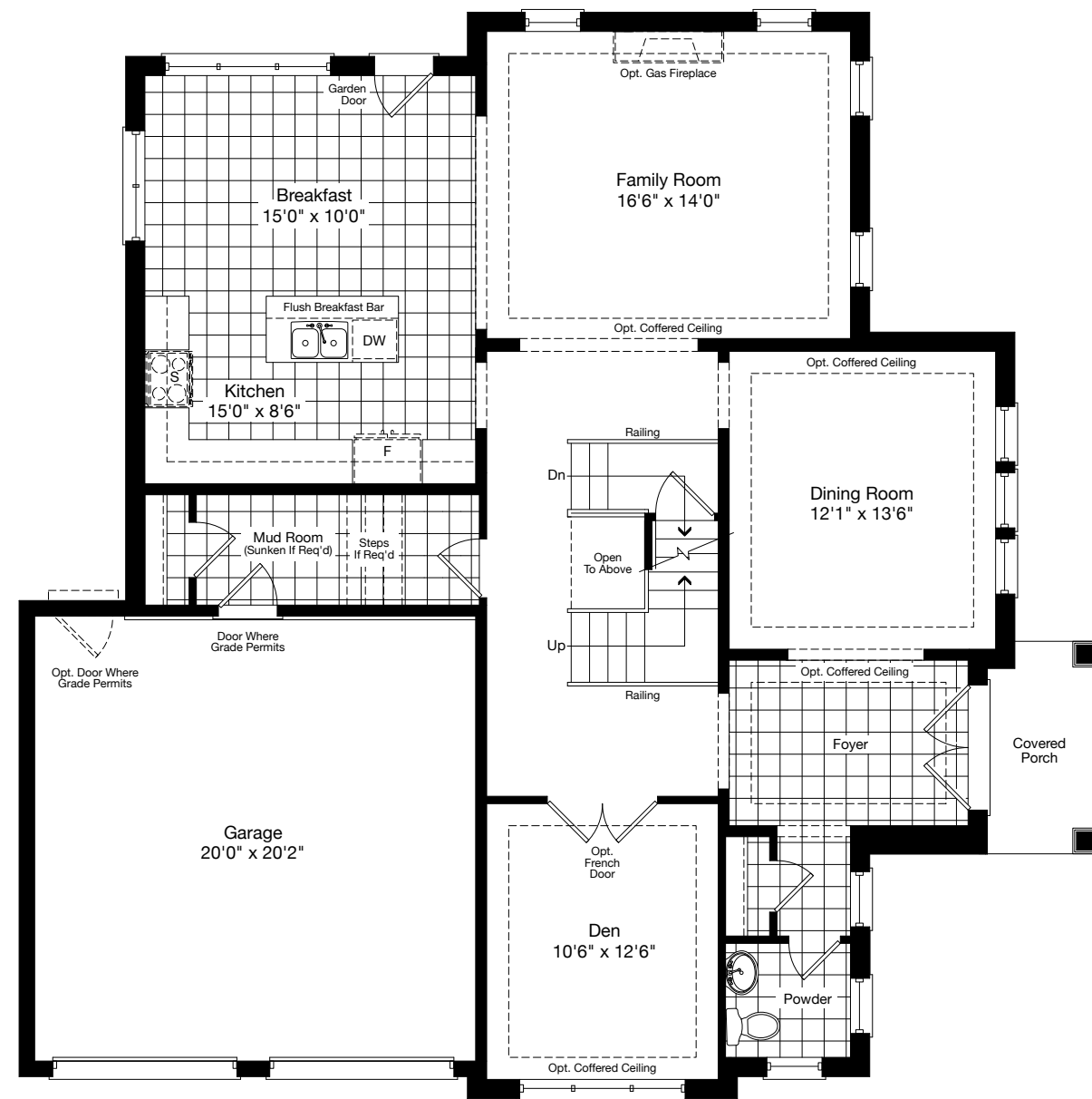
GROUND FLOOR ELEVATION A
