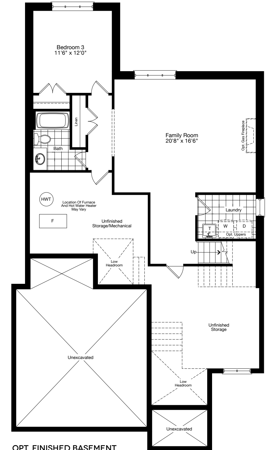
OPT. FINISHED BASEMENT ELEVATION A & B - 866 SQ.FT
