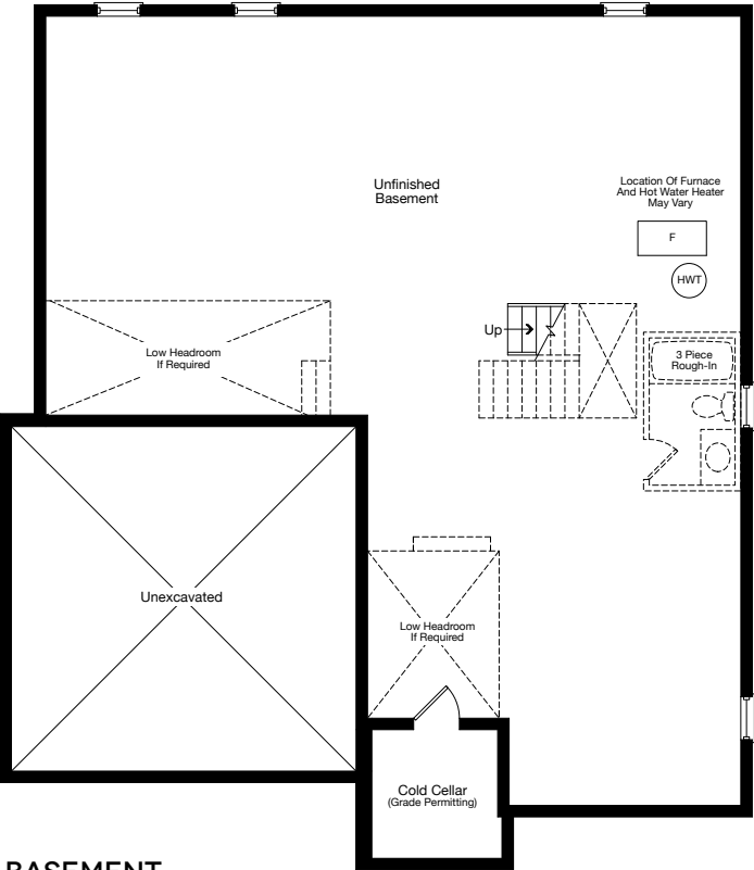
BASEMENT ELEVATION A & B
