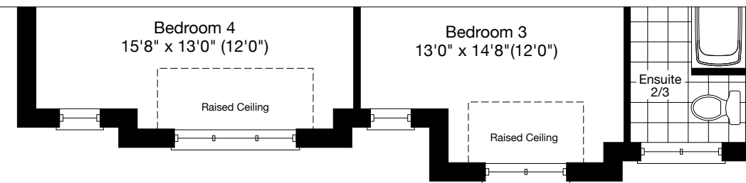
PARTIAL SECOND FLOOR ELEVATION B
